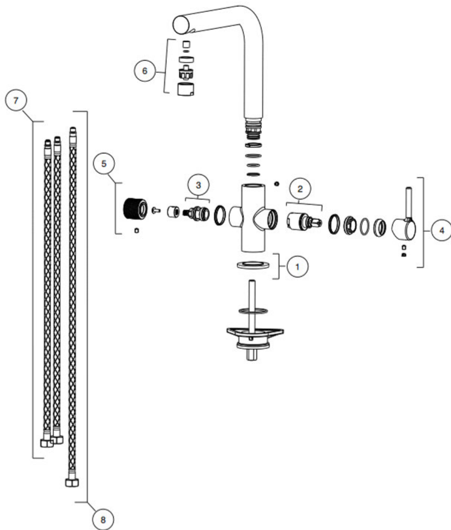
Lina Filter 2.0 Tap L Swivel CHR
